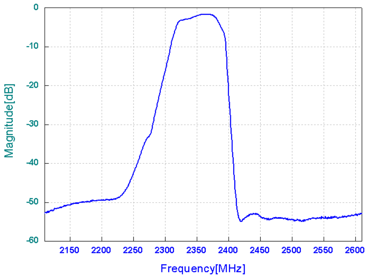
Frequency Response
